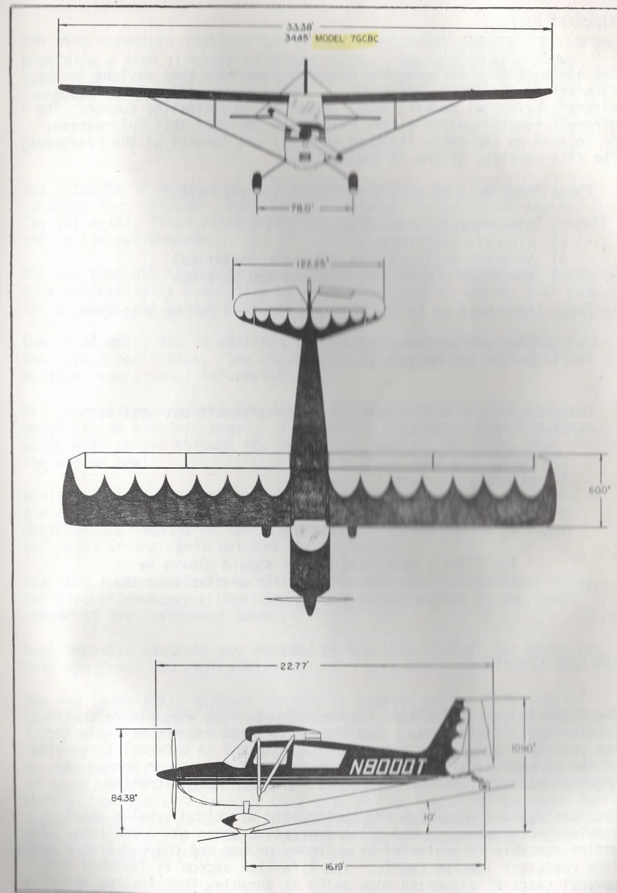
FIGURE 6-2 CITABRIA THREE-VIEW
